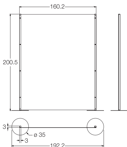
② Cloison fixe
