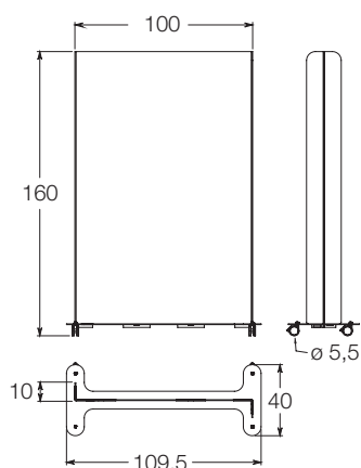
① Cloison mobile
